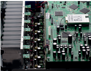
Discrete built amplifier stage
